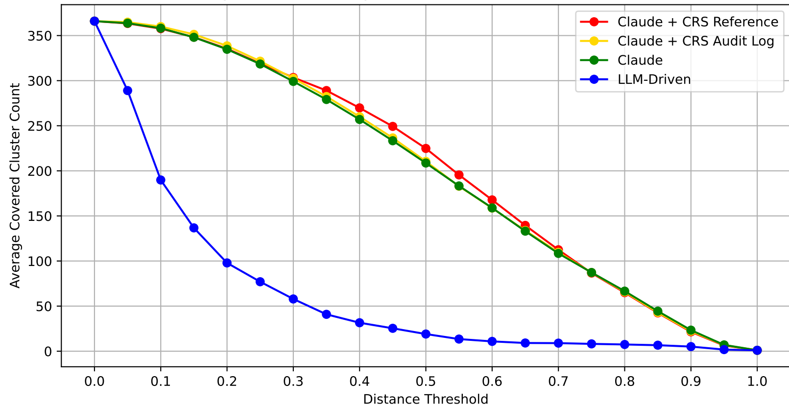
Average Cluster Coverage vs Distance Threshold (Seeds 1-100)
